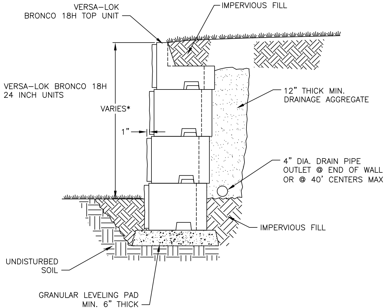
BRONCO 18H UNREINFORCED RETAINING WALL 24 INCH UNITS SCALE: NONE
